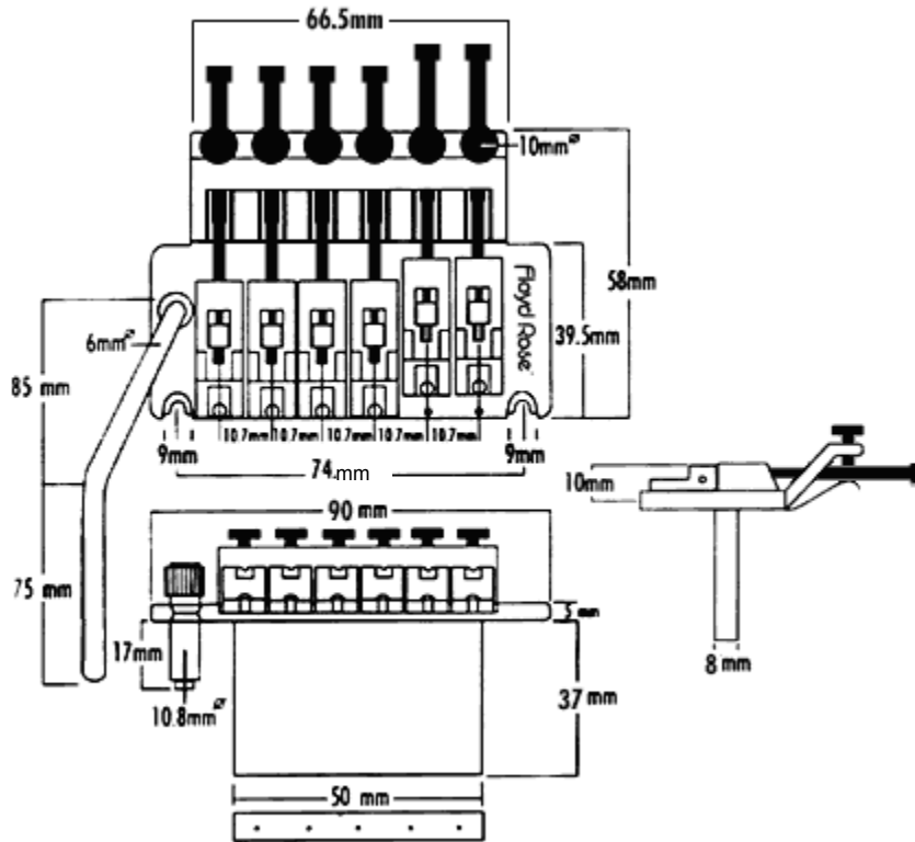
Dimensions in Millimeters
